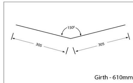
VALLEY GUTTER
