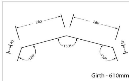
RIDGE CAP
