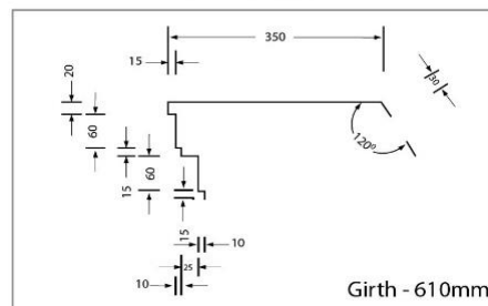
BARGE CAP
