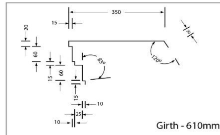
GABLE CAP
